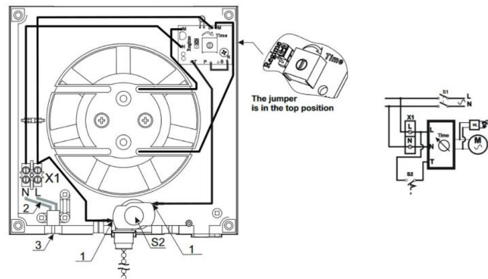
Fan with timer switch and pull-cord switch (type LZ) in diameter 100,125
